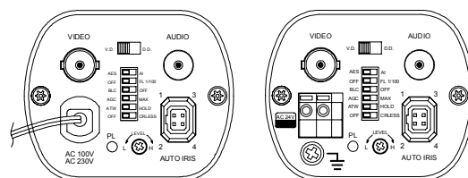
Rear Panel
